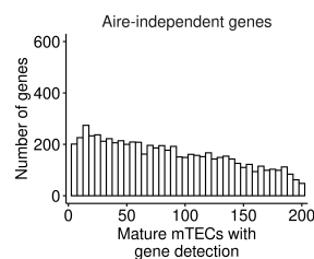
Plot VII: Histogram and heatscatter of genes stratified by Aire regulation.
