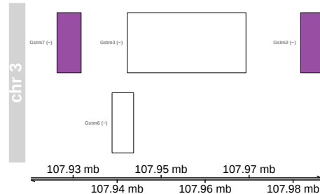
Plot XXIX: Other related genes. Supplementary 8B.
