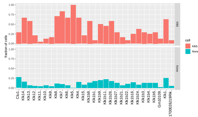
Plot XXXIII: Kik expression. Supplementary S9.
