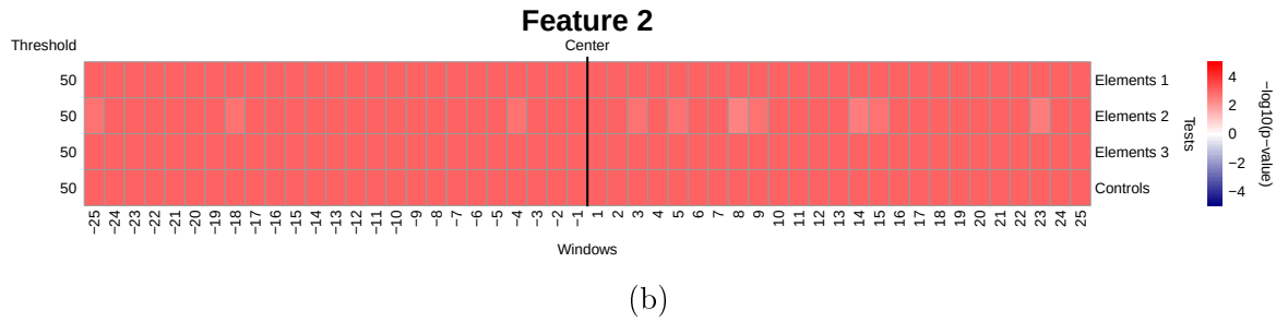
Figure 10: Summary plots of IWT results about the center of symmetry of the distributions of the different region datasets being equal to 1, grouped by (a) Feature 1 and (b) Feature 2.
