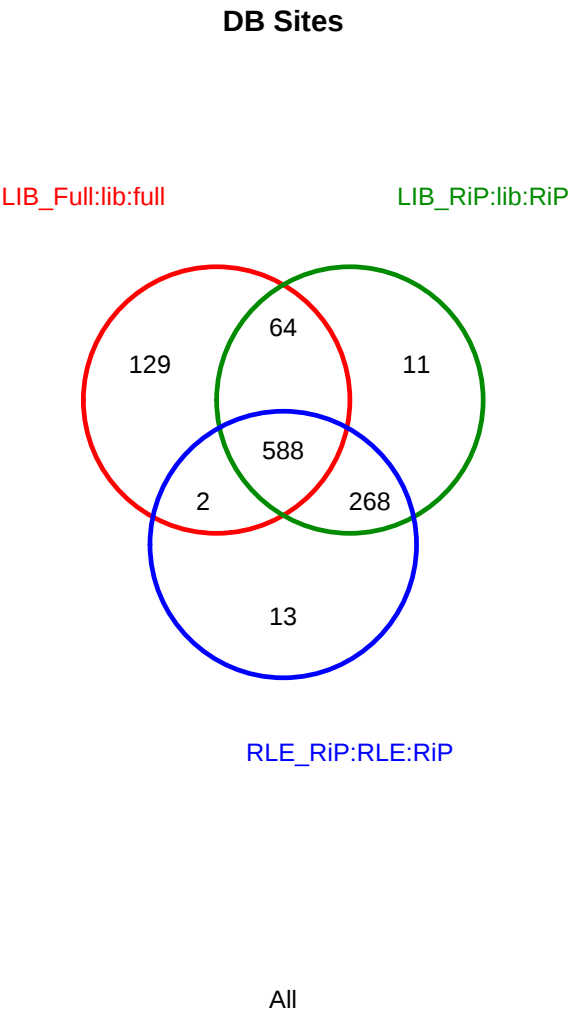
Figure 22: Venn diagram showing overlapping differentially bound sites identified in analyses using library-size normalization with full and reads-in-peaks library sizes, as well as RLE normalization using reads-in-peaks.
