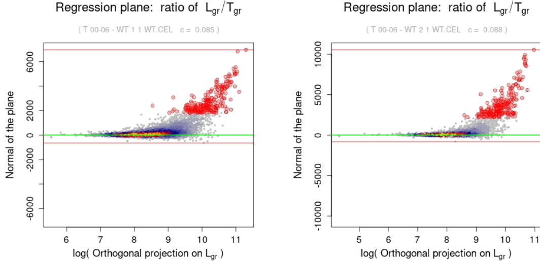
Figure 2: Two rounds of total least squares regression ( tls ). The resulting plane is shown exactly from the side and is colored green. The x-axis of those plots is chosen as the orthogonal projection on L in logarithmic scale. The y-axis is the normal of the plane. The second round of tls is performed without the 5% largest residues of the first round, depicted in red. Red lines indicate maximal residues.
