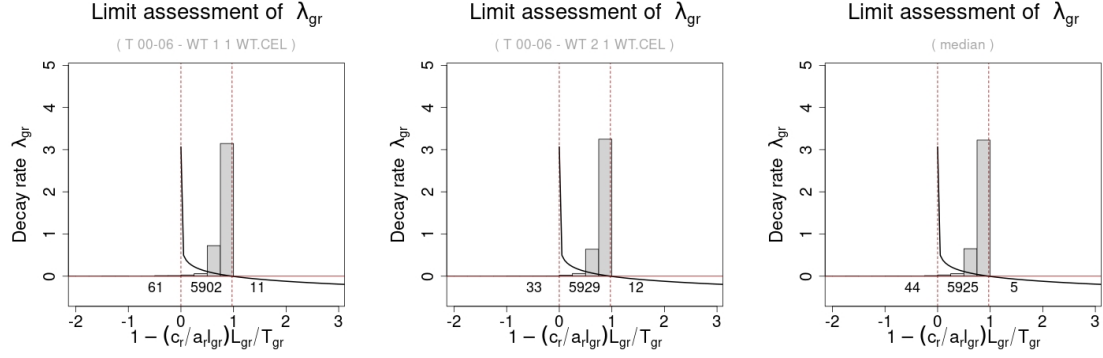
Figure 4: Dependency of 1-cL/T to the resulting decay rate. Reasonable decay rates can only be obtained for 1-cL/T values between the two dashed lines. All others will yield NAs.
